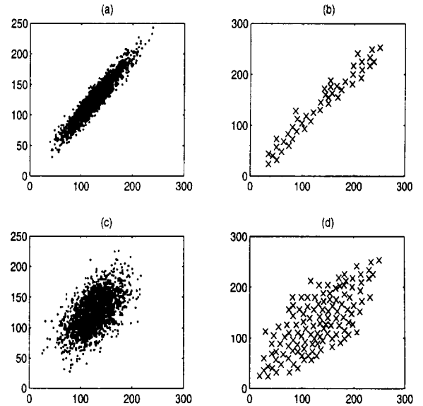
Figure 2: Adaptation of RDLZ Codebook. (a) Source distribution at time t_1 , \rho = 0.9 , (b) codebook at time t_1 , (c) source distribution at time t_2 , \rho = 0.6 , (d) Codebook at time t_2 . Results: RDLZ gives SQNR = 27.1 dB, rate = 2.3986; TSVQ gives SQNR = 27.1 dB, rate = 2.683
