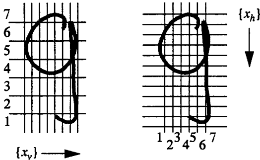
Figure 4: Generation of the sequences of feature vectors \{x_v\} and \{x_h\} , illustrated by the number „9“
