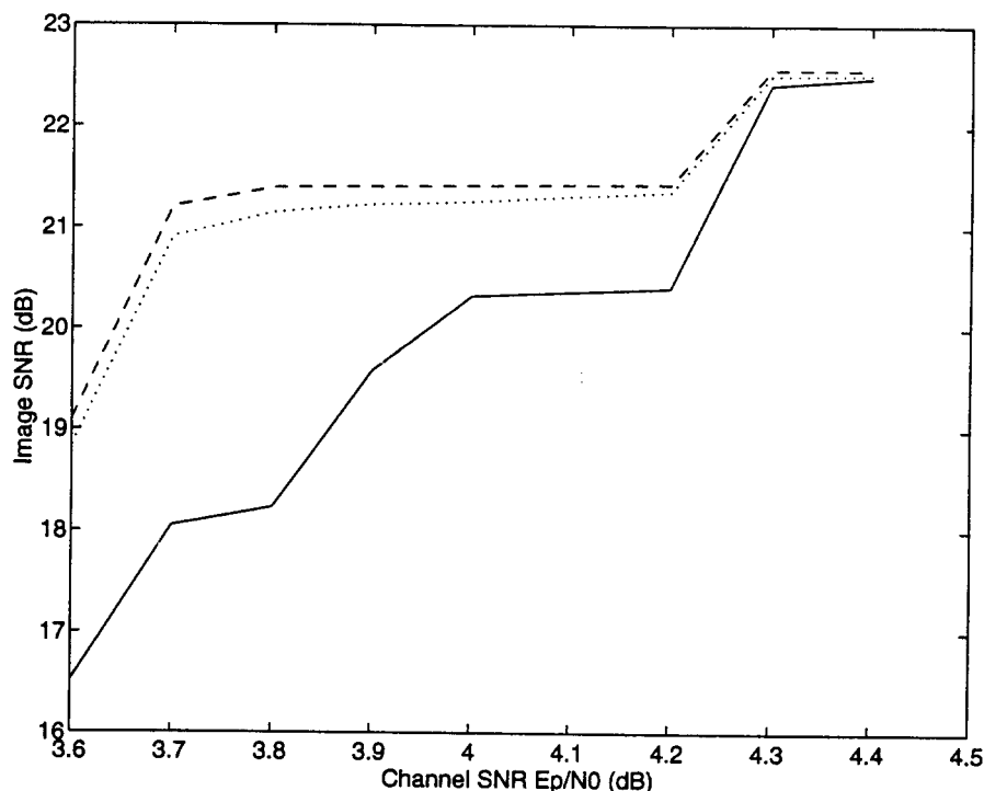
Figure 6: Image SNR vs. Channel SNR
