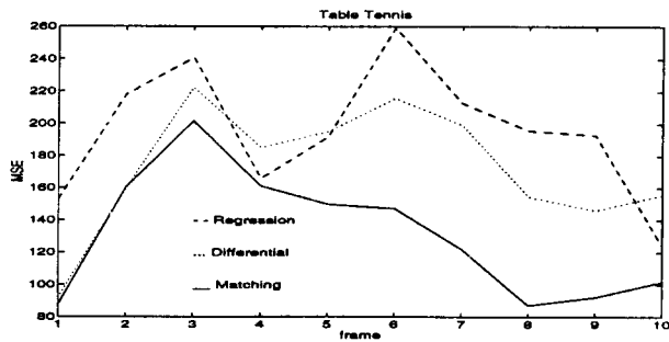
Figure 2: Comparison of the three approaches to global motion estimation: matching technique, differential technique and regression on a local motion field.
