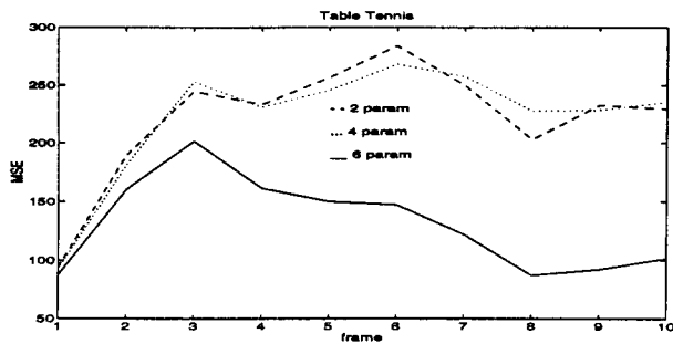
Figure 3: Comparison of the respectively 2, 4 and 6 parameters model for camera motion.
