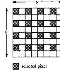
Figure 1: The selected pixels of 4 to 1 subsampling
