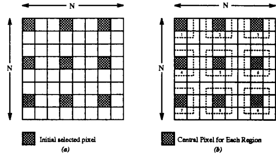
Figure 2: Adaptive pixel selection (a) 9 selected pixels. (b) the selected pixels in (a) are considered as the central pixel for each region, the dotted lines indicate the neighbor pixels for respective central pixels in each region.
