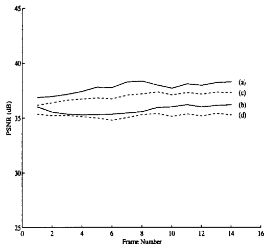
Figure 5: PSNR results for "helicopter" image sequence: proposed video coding at 0.1 bits/pel (a) and 0.05 bits/pel (b) and MC-DCT video coding at 0.1 bits/pel (c) and 0.05 bits/pel (d).
