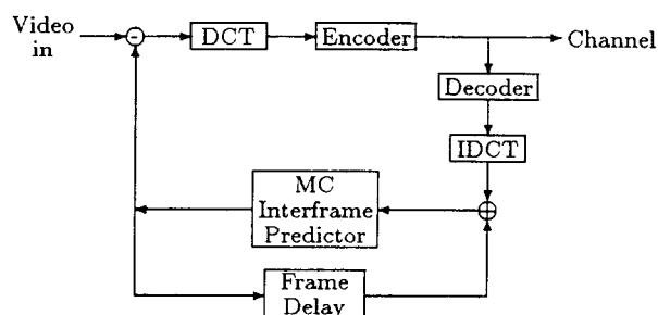
Figure 1: Basic structure of MC-DCT video coding.
