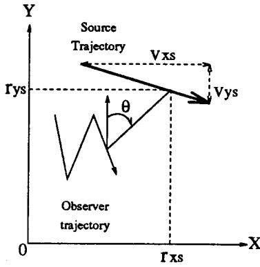
Figure 1: Source-Observer encounter.
