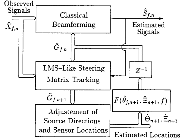
Figure 2: The block diagram at frequency f .
