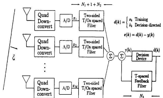
Figure 1: Multichannel adaptive equalizer.
