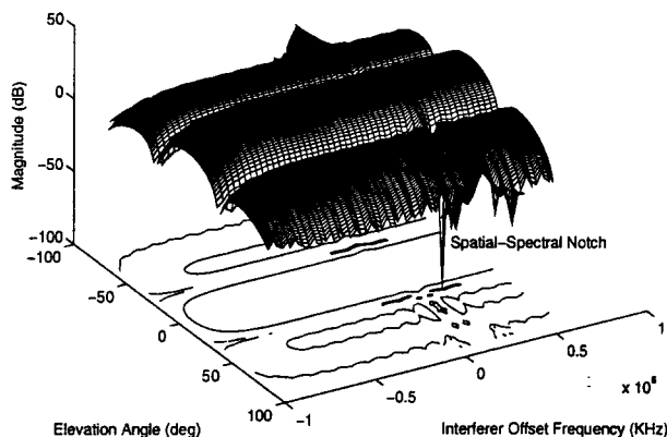
Figure 2: Beampattern for MAEQ with M = 4 and N = 30 with an interferer at 50^\circ elevation.
