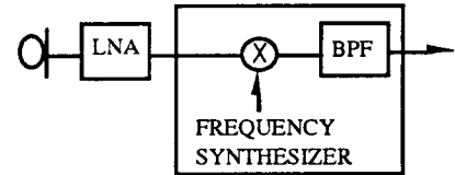
Figure 2. Dehoppping system (at each sensor)
