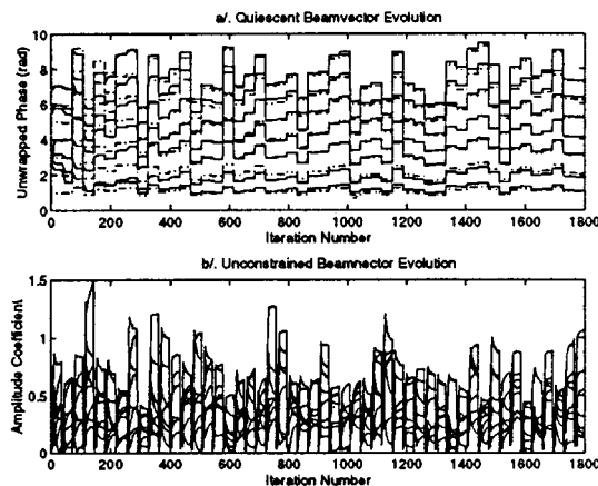
Figure 6. Coefficients Evolution
