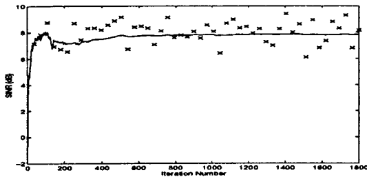
Figure 4. SINR Evolution
