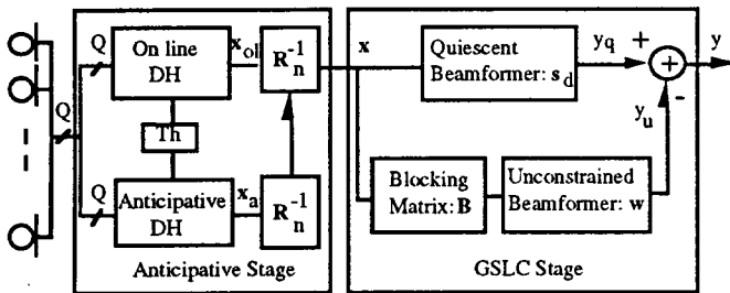
Figure 1. Frequency Hopping Receiver
