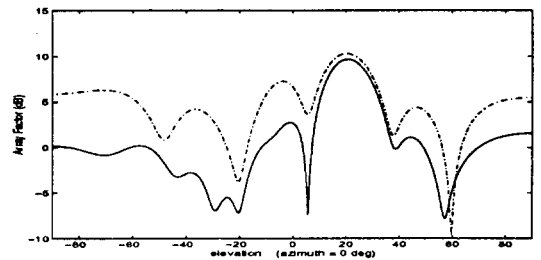
Figure 3. Array Factor
