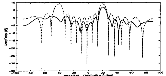
Figure 7. Array Factor
