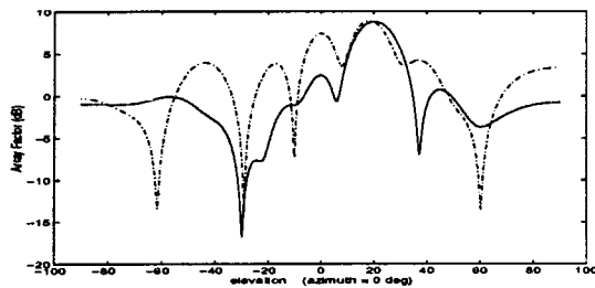
Figure 5. Array Factor
