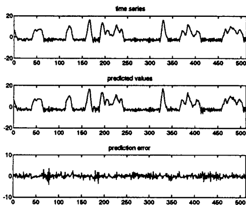
Figure 4: Tree-based 1 step forward prediction and prediction errors
