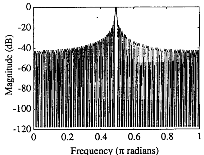
Fig. 8. Direct DFT Analysis Response
