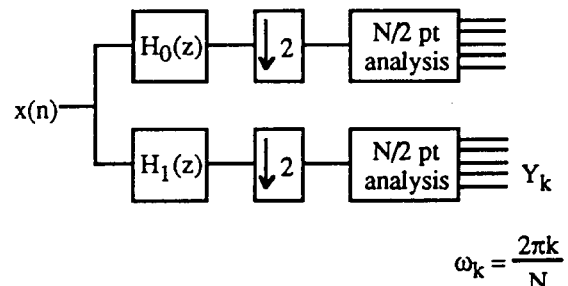
Fig. 2. Subband Spectral Analysis
