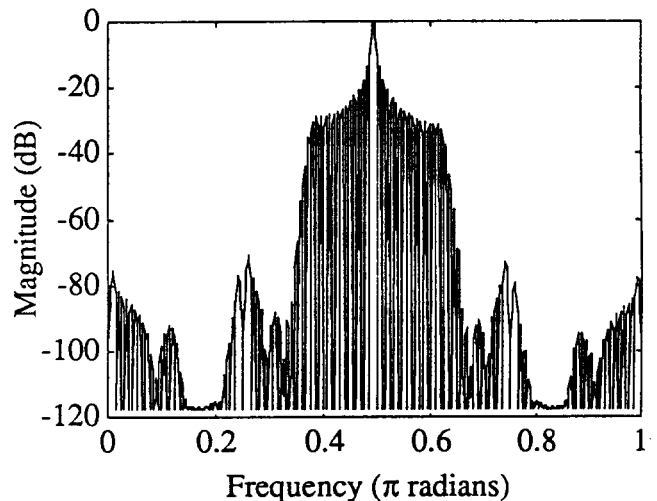
Fig. 7. Alias-Canceled Subband Analysis Response
