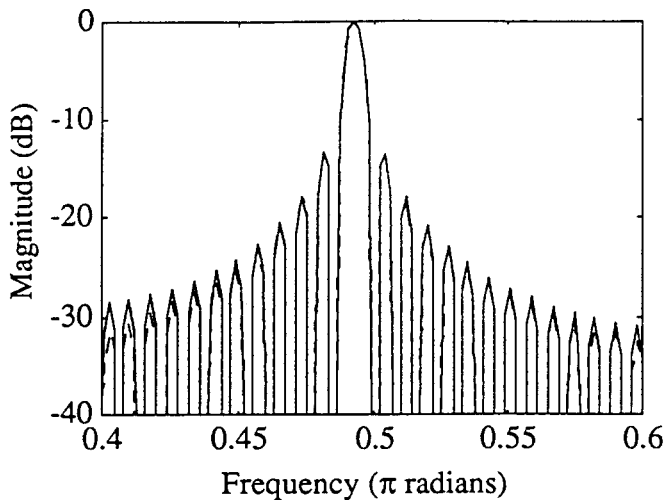
Fig. 9. Comparison of 256 pt direct DFT (dashed) and Alias-Canceled 32 pt subband DFT (solid) Analysis Responses
