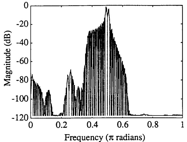
Fig. 6. Non Alias-Canceled Subband Analysis Response
