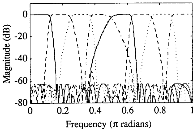
Fig. 5. 8-band QMF Frequency Response
