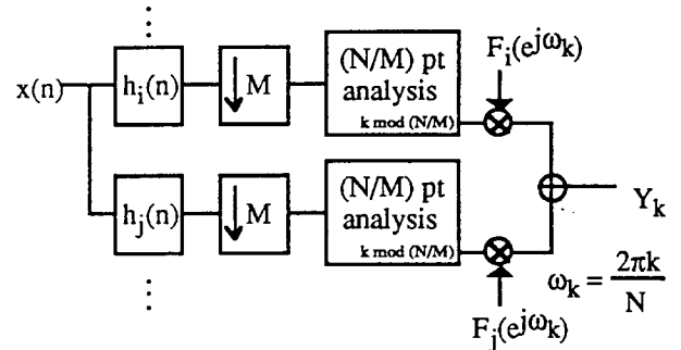
Fig. 3. Alias-Canceled Subband Spectral Analysis
