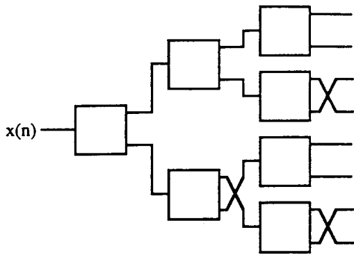
Fig. 4. 8-band QMF tree structure
