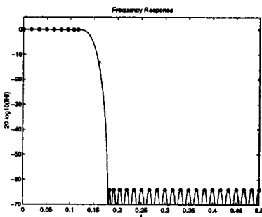
Figure 3: The frequency response for example 2.
