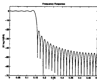
Figure 2: The frequency response of the best unconstrained L_2 filter.
