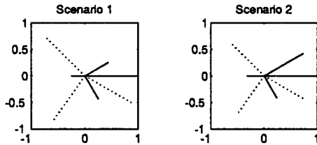
Figure 5: Scenario 1 and 2. Desired signals (solid) and co-channel interferers (dotted). The line lengths are proportional to the square root of the power impinging from each direction. The antenna is located at the origin.
