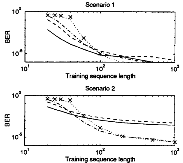
Figure 6: BER 1 for scenario 1 and 2: MIB-DFE(solid), SBE-LS with one (dashed), two (dash-dotted) and four (dotted) beamformers and GB-DFE(x). SNR=SIR=4dB.
