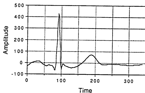
Fig. 4 Reconstruction after compression
