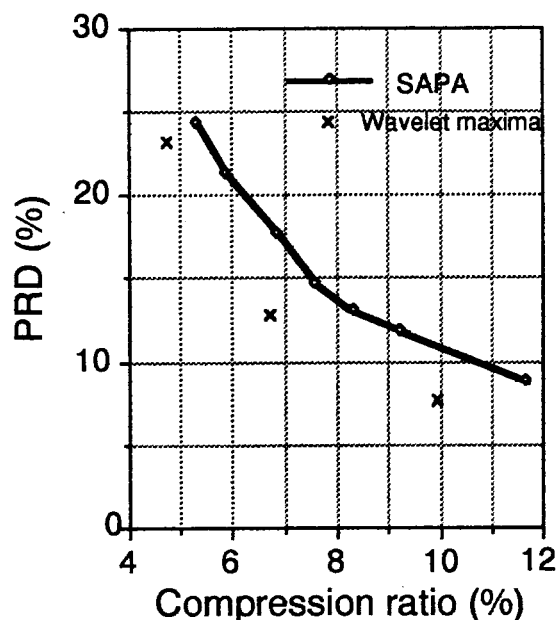
Fig. 5 Compression ratio vs reconstruction error
