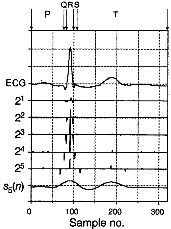
Fig. 1 Multiscale peak analysis of an ECG waveform
