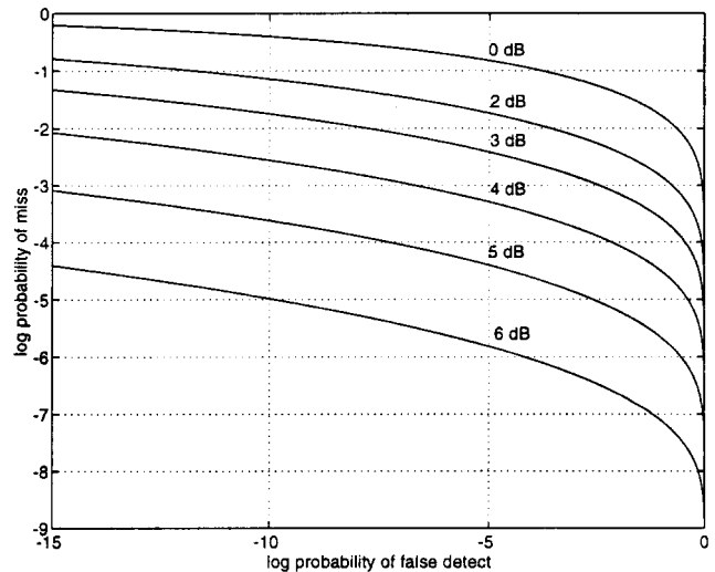
Figure 2. \log_{10} P_m vs. \log_{10} P_{fd} for the decision rule (5) assuming K = 1 , N = 10 , and \text{SNR} = 15 dB. Each plot corresponds to a different power level for the new interferer.
