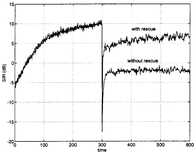
Figure 1. SIR vs. time for for the LMS algorithm, and the LMS algorithm with a rescue at time iteration 300. N = 10 , K = 6 , \text{SNR} = 15 dB, A_k/A_1 = 3 , k = 2, \dots, 6 , A_7/A_1 = 15
