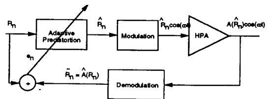
Figure 4: Transmitter
