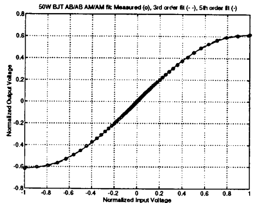
Figure 2: BJT class AB AM Char.
