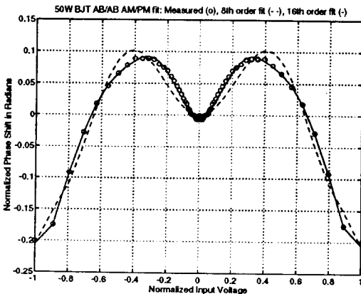
Figure 3: BJT class AB PM Char.
