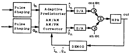
Figure 1: Digital Transmitter
