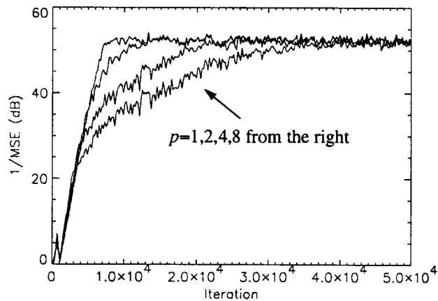
(a) for a colored noise generated through an 8-order IIR filter, \mu_1 = 0.25 .
