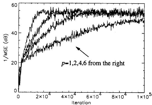
(b) for a colored noise generated through a 4-order IIR filter, \mu_1 = 0.5 .
