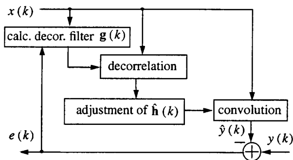
Figure 1. Block diagram of conventional Projection algorithm
