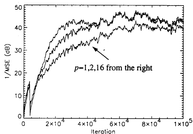
(c) for a speech signal, averaged 50 trials, \mu_1 = 0.5
