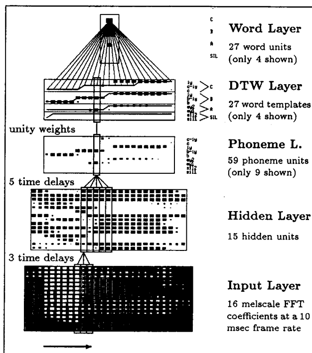
Figure 1: The MS-TDNN recognizing the excerpted word 'B'. Only the activations for 'SIL', 'A', 'B', and 'C' are shown.
