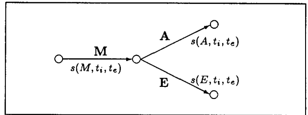
Figure 4: The fully constrained search viewed as a graph search problem. The goal is to find an optimal path through the graph. Each transition corresponds to one letter. The partial score of a transition depends on t_i and t_e .
