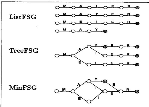
Figure 3: Different types of graphs to represent the strings MAYER , MAIER , MEIER , MAY .
