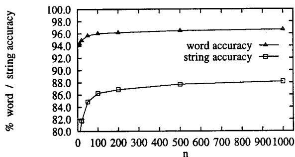
Figure 2: String and word accuracy as a function of the size of the n -best list.
