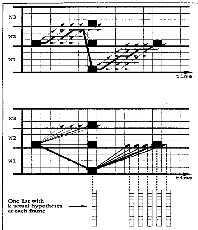
Figure 5: Top: Conventional DTW search technique. The matrix contains the prohibitive amount of 57,713 word models, one for each letter in the minFSG. Bottom: Two level search with only one word model for each letter in the alphabet, but an expensive precomputation of partial scores. At each frame, a list with the active search hypotheses is kept.
