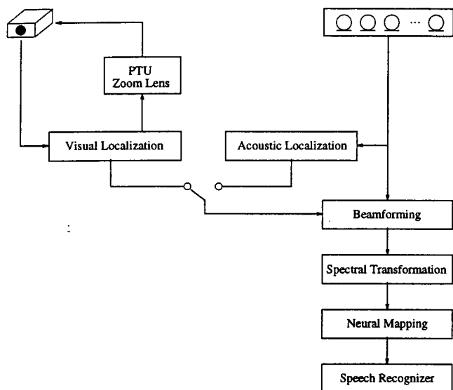
Figure 2. Acoustical and visually guided beamforming.
