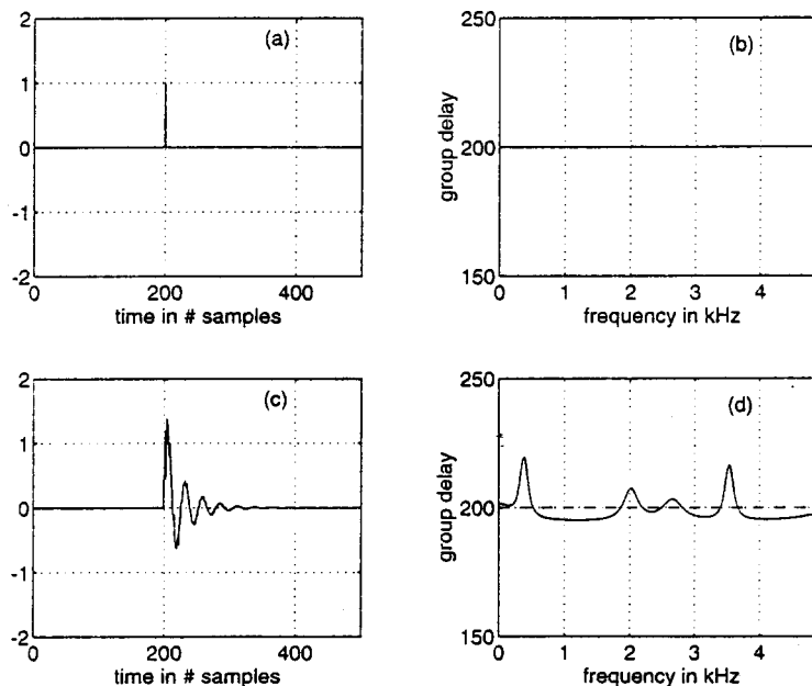
Figure 1. (a) Delayed unit sample sequence. (b) Group delay function for delayed unit sample sequence in (a). (c) Response of an all-pole filter for the unit sample sequence in (a). (d) Group delay function for the signal in (c).
