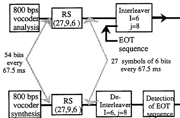
EDAC of the speech mode of HF-ECCM system
