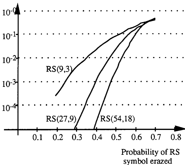
Probability of NO RS Decoding
