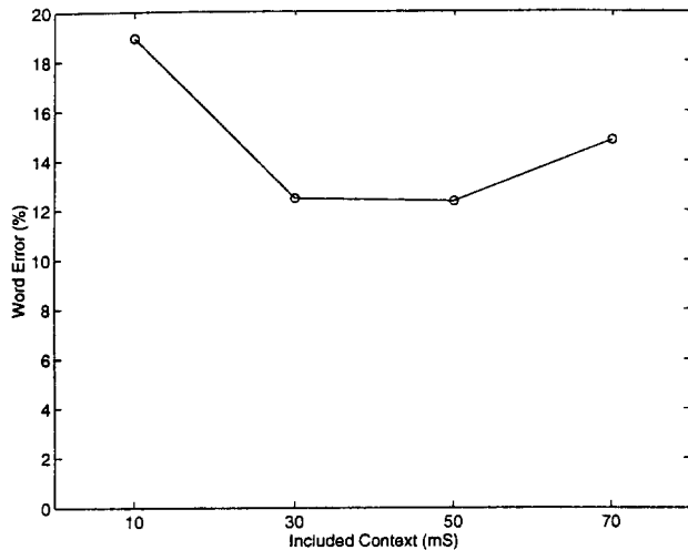
Figure 4. Word error vs. context (1024-leaf tree).
