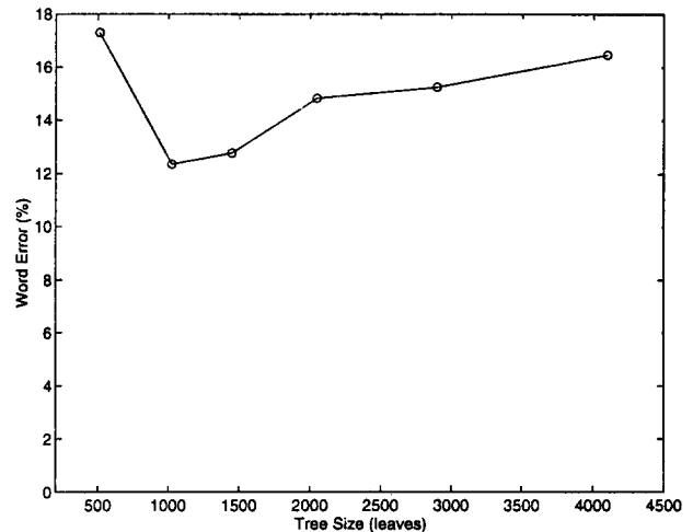
Figure 5. Word error vs. tree size (50-ms context).
