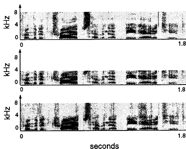
Figure 6: a) Spectrogram of the original speech, b) spectrogram of downsampled signal and c) recovered spectrogram.
