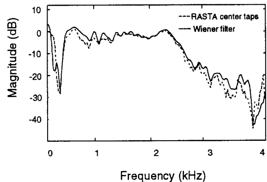
Figure 4: Wiener filter response and RASTA center taps.
