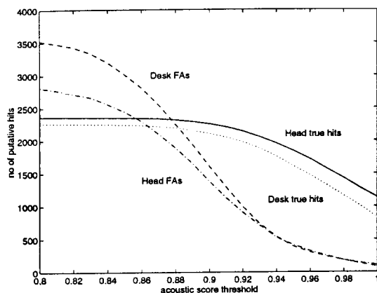
Figure 3. Nos of putative hits versus threshold.
