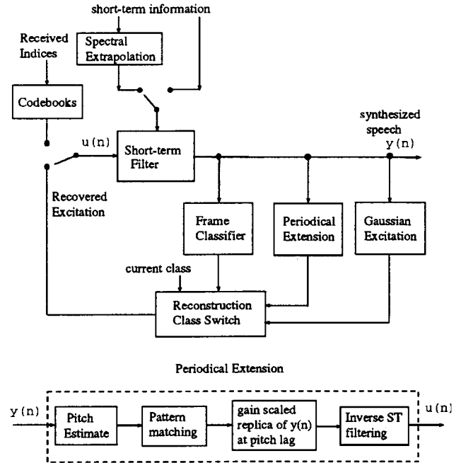
Figure 1: Packet Reconstruction Model
