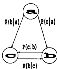
Figure 1: Example of a bi-gram network
