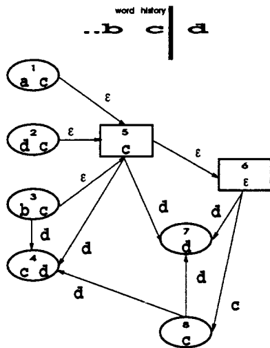
Figure 3: Portion of a 3 rd order VNSA network
