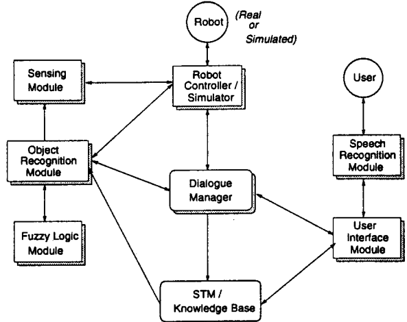
Figure 2: System Architecture
