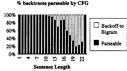
Figure 3: Percentage of backtraces covered by the SCFG
