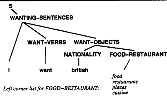
Figure 2: Prefixes and Left-Corner lists
