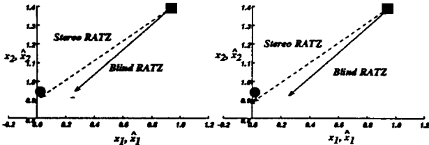
Figure 3. Comparison of compensation vectors obtained using stereo RATZ and blind RATZ. Filled circles and filled squares denote the locations of clean speech and uncompensated degraded speech, respectively.
