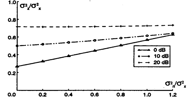
Figure 2. Effect of noise on the variance of z . The curves are plotted for three values of the relation \mu_x - \mu_n , 0, 10, and 20 dB.
