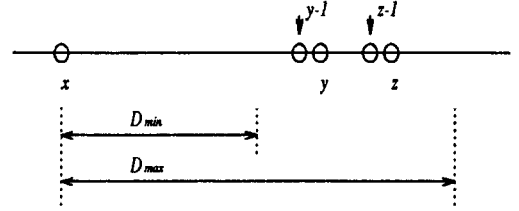
Figure 2: A section of an example utterance. x, y , and z are possible beginning points, while y-1 and z-1 are ending points corresponding to x .
