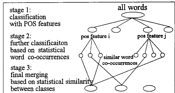
<fig. 4> The three-stage hierarchical word classification algorithm
