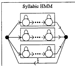
<fig. 2> The syllable net composed of syllabic HMM
