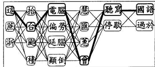
<fig. 3> A partial listing of an example word lattice. Note: The correct word string here is "這台電腦會聽寫國語" (This computer can be dictated using Mandarin.)"
