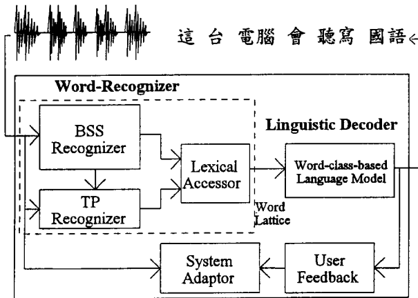
<fig. 1> The overall system block diagram
