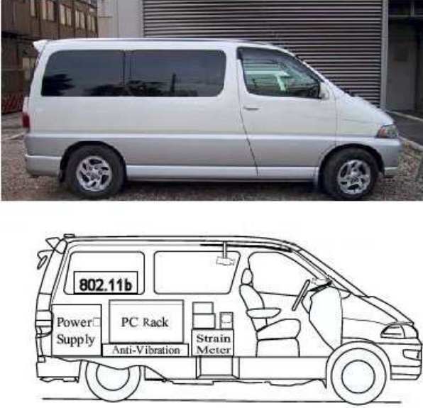
Fig. 1. Data collection vehicle used during the experiment.
