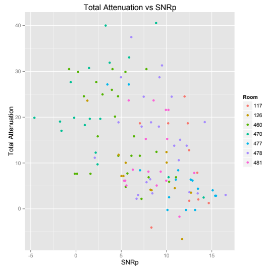
Figure 5. Total Attenuation vs SNRp.
