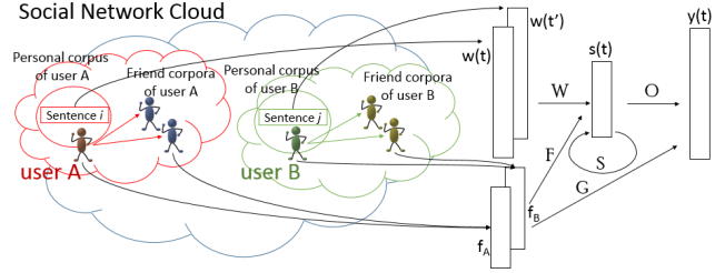
Fig. 1: The scenario for the proposed approach. When training with sentence i from user A, the user feature fed into the RNNLM can be produced by either topic distribution of user A's personal corpus or searching over user A's personal / friends corpora for sentences with topic distributions closest to this sentence i .
