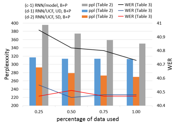
Fig. 4: Perplexity (PPL) and word error rate (WER) for different sizes of personal corpus for the model adaptation approach ( (c-1) RNN/model, B+P ) and the proposed approaches ( (d-1) RNN/UCF, UD, B+P and (d-2) RNN/UCF, SD, B+P ). The horizontal axis is the percentage of the original personal corpora used ( 1.00 on the right is for the data in Tables 2 and 3 ).
