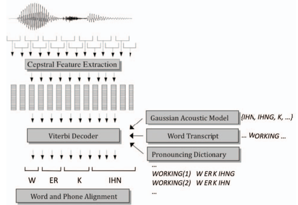
Fig. 2. Procedure for “g-dropping” detection using forced alignment.
