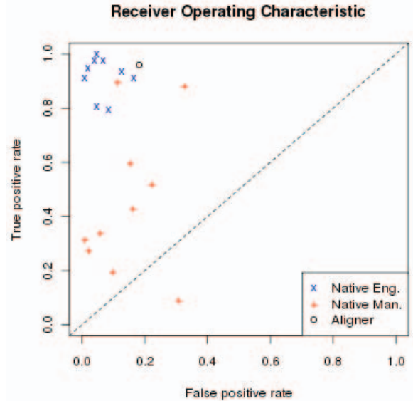
Fig. 5. True and false positive rates of English listeners, Chinese Listeners, and the alignment method, using the majority vote of the English listeners as the gold standard and the presence of “g-dropping” as the positive.
