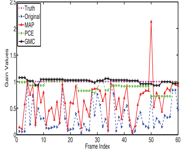
Fig. 5. Estimation of constant gain parameter.
