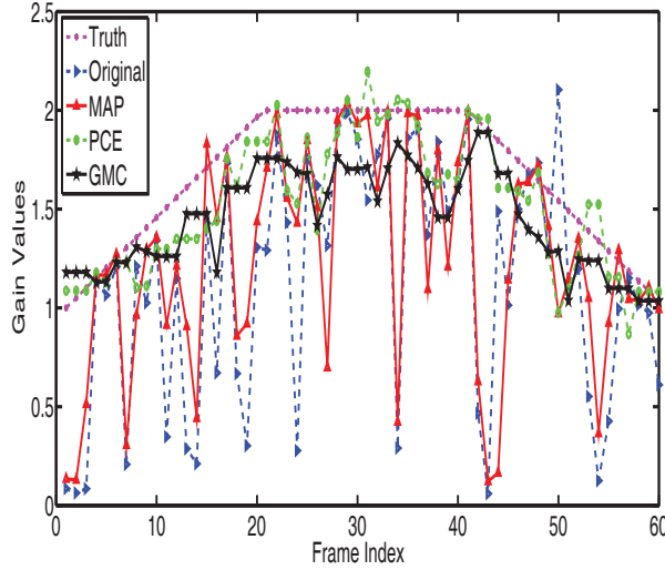
Fig. 6. Estimation of fading gain parameter.
