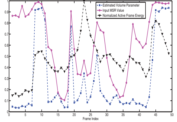
Fig. 2. Gain Estimation Problem Reasons: Low Input MSR and Low Active Frame Energy.
