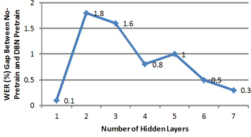
Fig. 1. Word error rate gap in percentage points between the system without pretraining and that with DBN pretraining.
