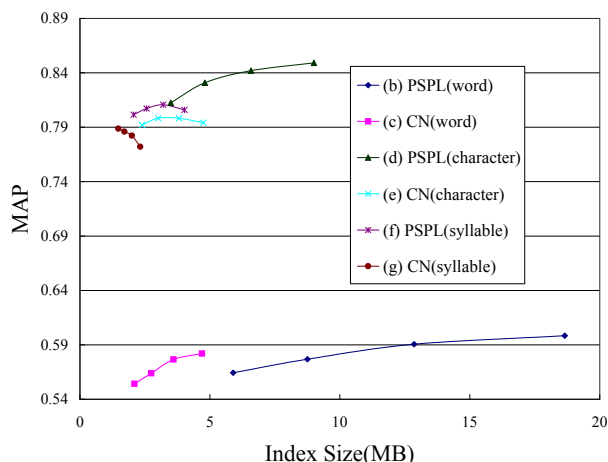
Fig. 3. The tradeoff between MAP and index size for the different approaches considered.
