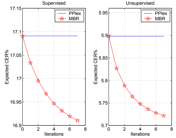
Fig. 1. MBR criterion on bnmdev06, bcmdev05 and eval06 for supervised and unsupervised adapted LMs using PP and MBR.
