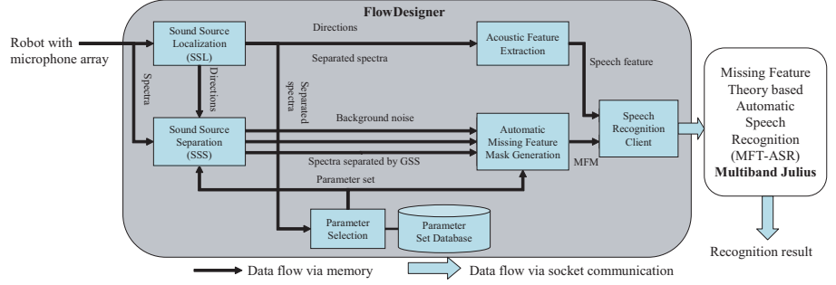
Fig. 3. Overview of the real-time robot audition system
