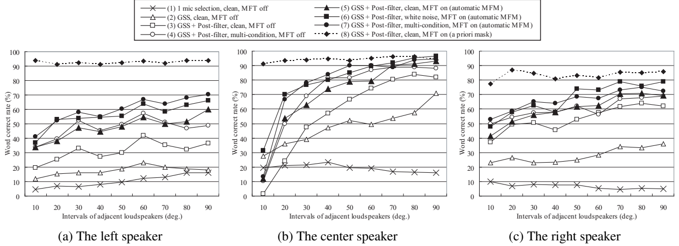
Fig. 4. Word correct rates of three simultaneous speakers with our system
