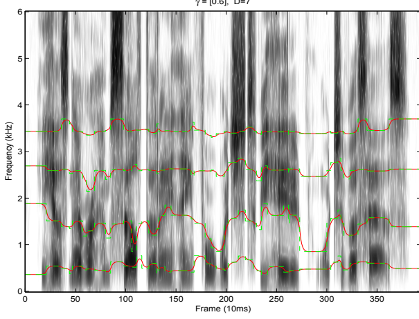
Fig. 8. The f_1/f_2/f_3/f_4 VTR frequency trajectories (smooth lines) generated from the model for VTR target filtering using the phone sequence and duration of a speech utterance (SI1039) taken from the TIMIT database. The target sequence is shown as stepwise lines, switching at the phone boundaries labeled in the database. They are superimposed on the utterance’s spectrogram. The utterance is “ He has never, himself, done anything for which to be hated – which of us has ”.
