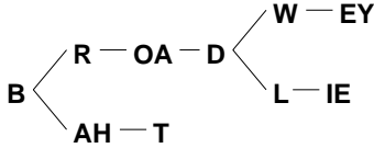
Figure 1: A simple pronunciation prefix tree (PPT) for a system using context-independent acoustic models.
